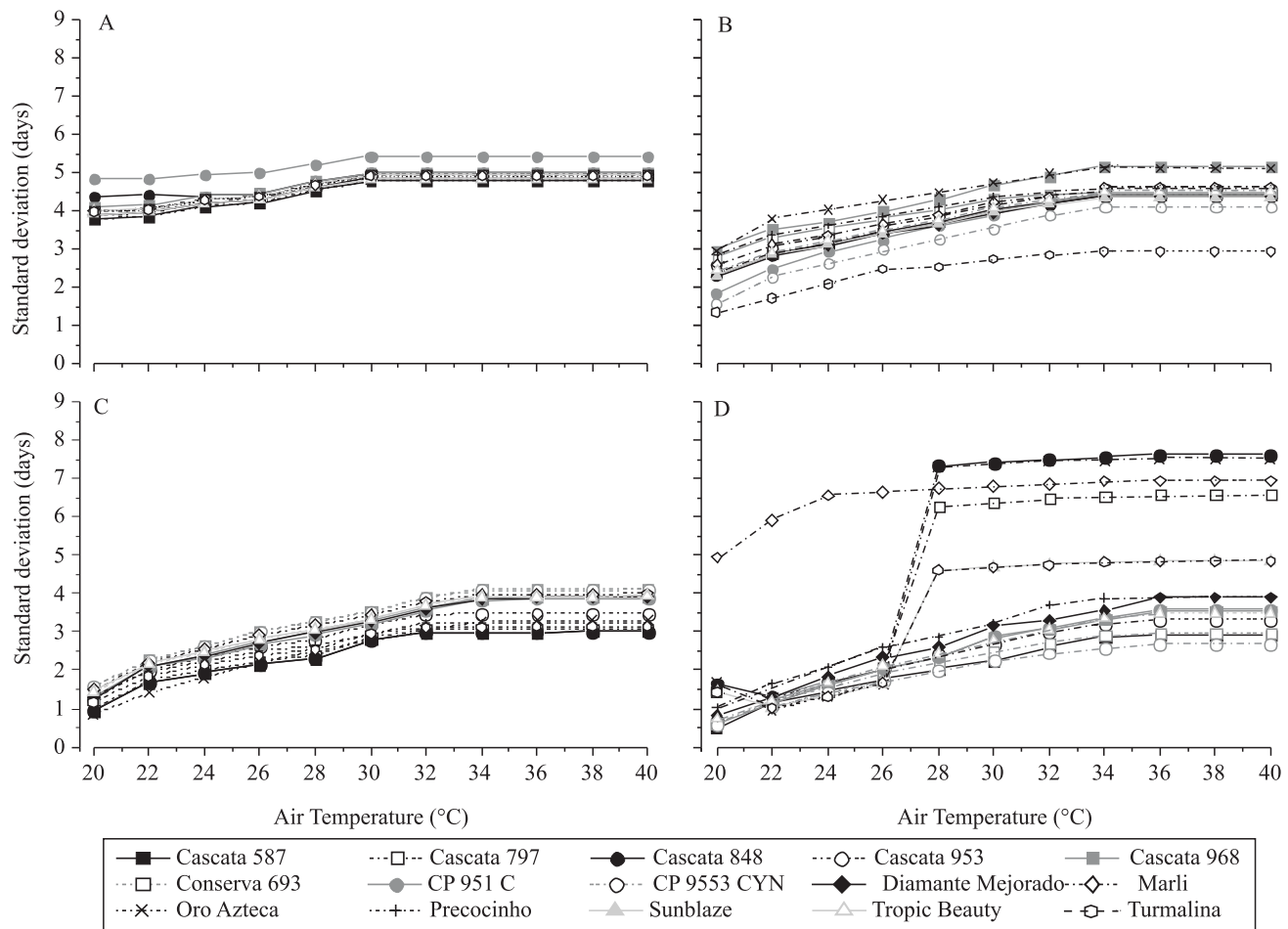
Figure 2. Maximum basal temperatures (TB) determined by the method of the lowest standard deviation for peach and nectarine cultivars, between pruning-sprouting (A), sprouting-flowering (B), flowering-fruitletting (C) and ripening (D) in Botucatu, SP, Brazil, between July 2006 and November 2009.
