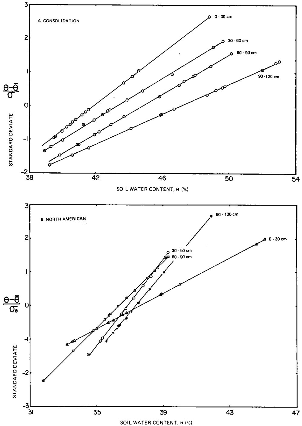
FIG. 1. Fractile diagram comparing water content at 0.3 bar soil water suction at different depths.
