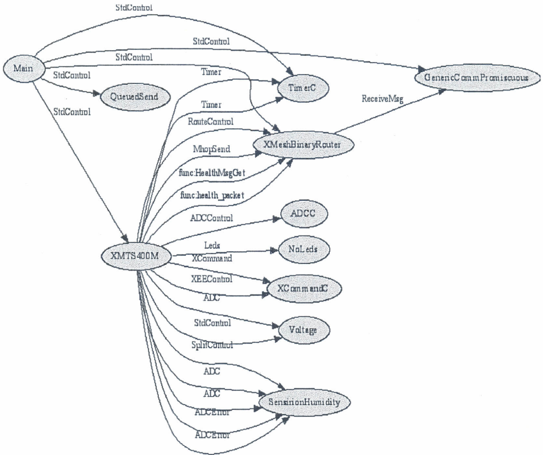
Fig. 6. XMTS400 components diagram to collect ambient temperature and relative humidity.
