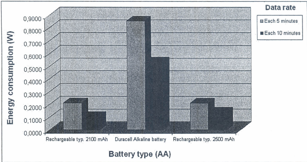
Fig. 7. Energy consumption for two sampling rates evaluated (5 and 10 min) in tree types of batteries.
