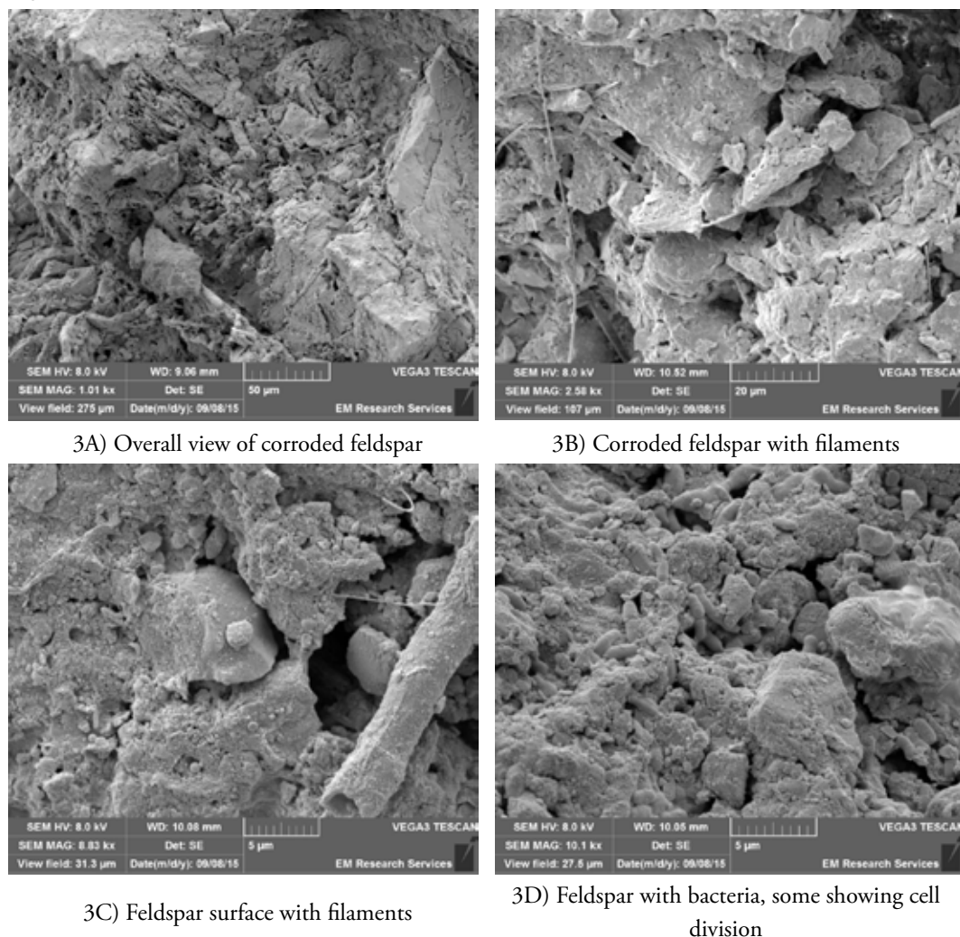
Figure 3 – Surface features of feldspar from soil developed on syenite, Triunfo, Pernambuco, Brazil.
