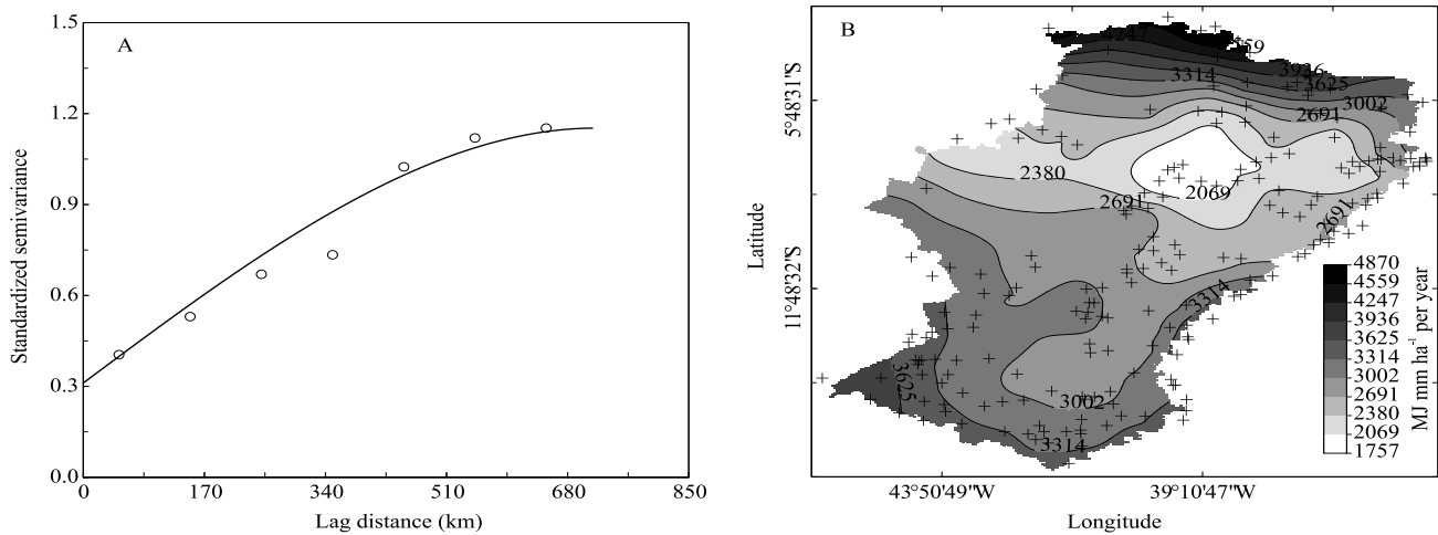
Figure 4. Annual semivariogram adjusted for erosivity values (A) and annual erosivity map for the semiarid region of Brazil (B). Daily series equal to or greater than 15 years of data.
