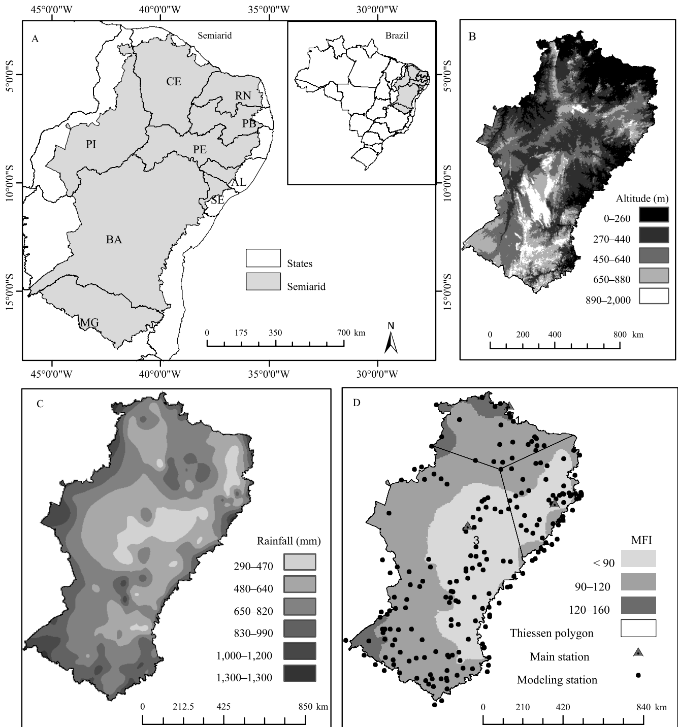
Figure 1. Location map of the Brazilian semi-arid region (A), altitude map (B), rainfall map (C), and annual map of the modified Fournier index (MFI) (D). Daily series equal to or greater than 15 years of data.
