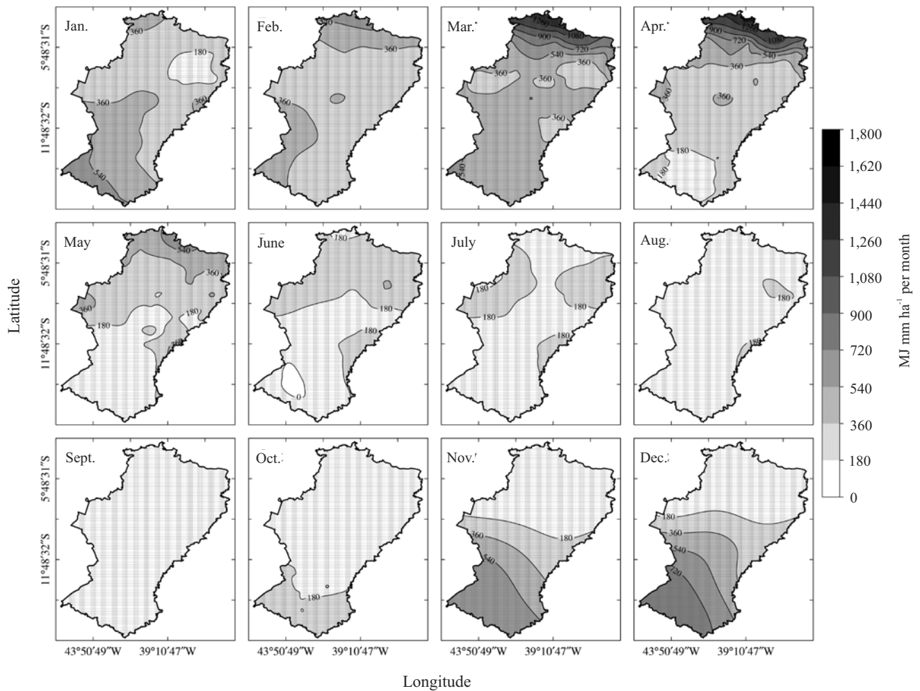
Figure 3. Spatial distribution of monthly mean erosivity in the semiarid region of Brazil. Daily series equal to or greater than 15 years of data.
