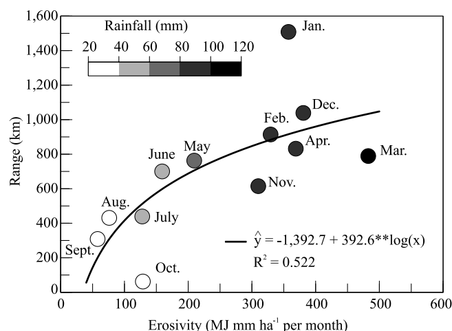
Figure 2. Correlation between monthly mean erosivity and range of spatial dependence for the semiarid region of Brazil. Daily series equal to or greater than 15 years of data.
