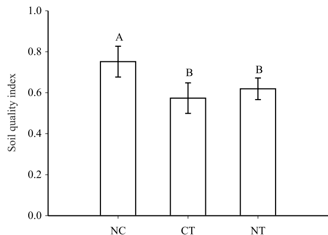
Figure 1. Soil quality index (SQI) according to the soil management systems, irrespective of the dataset. SQI means followed by equal letters do not differ by the Tukey's test, at 5% probability. NC, native area in Cerrado; CT, conventional tillage; and NT, no-tillage.
