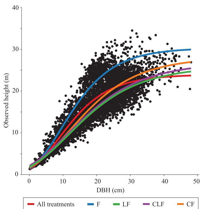
Figure 2. Gompertz's model-specific fitted curves to total data (All treatments) and to each production system – crop-forestry (CF), livestock-forestry (LF), crop-livestock-forestry (CLF), and monoculture forestry (F) – of Eucalyptus benthamii during seven years after planting in subtropical Brazil. DBH, diameter at breast height at 1.30 m above ground.
