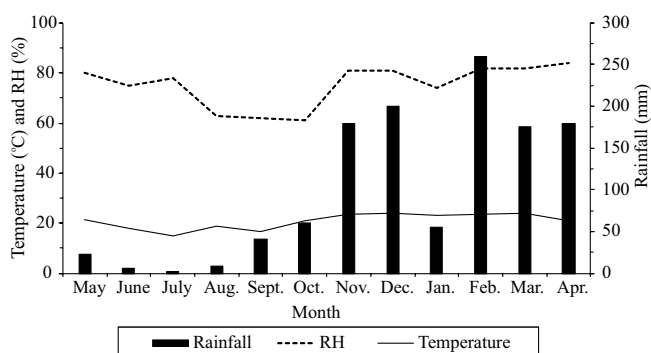
Figure 1. Monthly temperature, air relative humidity (RH), and rainfall, in the municipality of Diamantina, in the state of Minas Gerais, Brazil during the experimental period from May 2017 to April 2018. Source: Inmet (2020).
