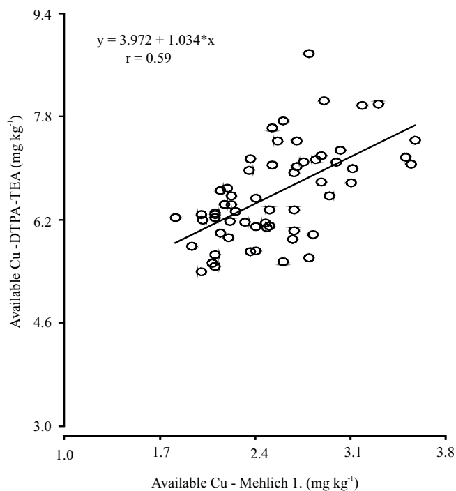
Figure 2. Relationship between the Mehlich-1 and diethylenetriaminepentaacetic acid-triethanolamine (DTPA-TEA) extractors, at pH 7.3, in determining available copper in the soil after cropping of soybean ( Glycine max ) cultivars. *Significant at 5% probability by the F-test.
