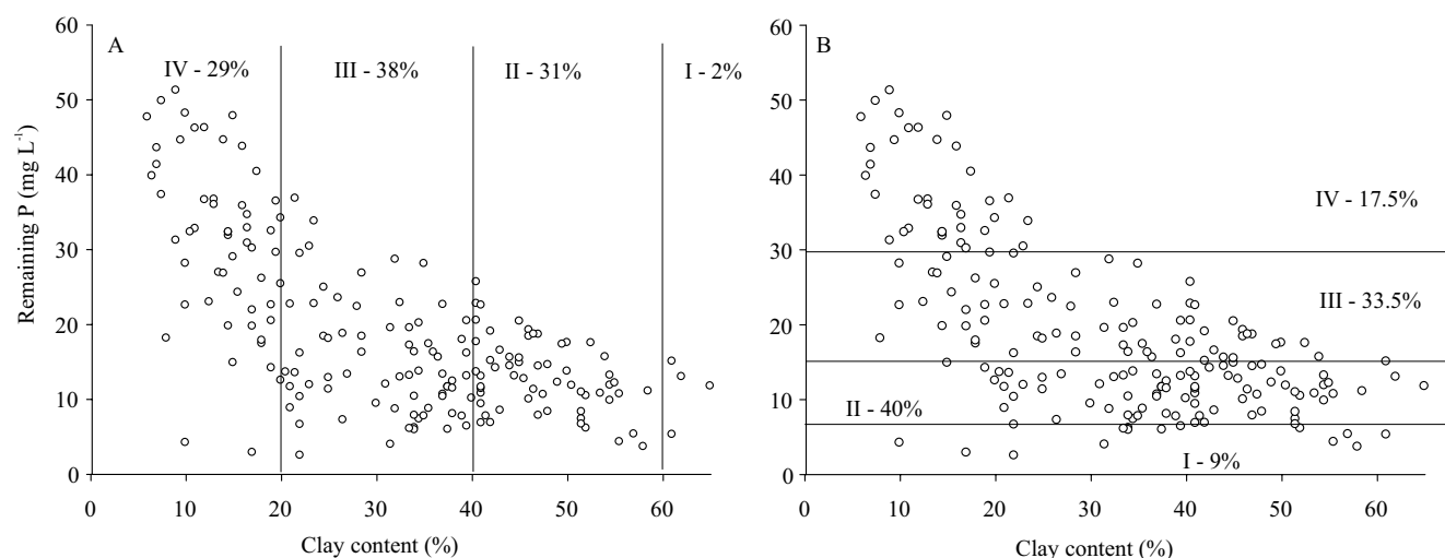
Figure 3. Sample distribution by the soil clay content index class (200 samples). Soil classification based on clay content: class I, > 60%; class II, 41–60%; class III, 21–40%; and class IV, <20% (Manual..., 2004); B, soil classification based on remaining P (60 mg L -1 ): class I, 0–7 mg L -1 ; class II, 7.1–15 mg L -1 ; class III, 15.1–30 mg L -1 ; and class IV, 30.1–60 mg L -1 .
