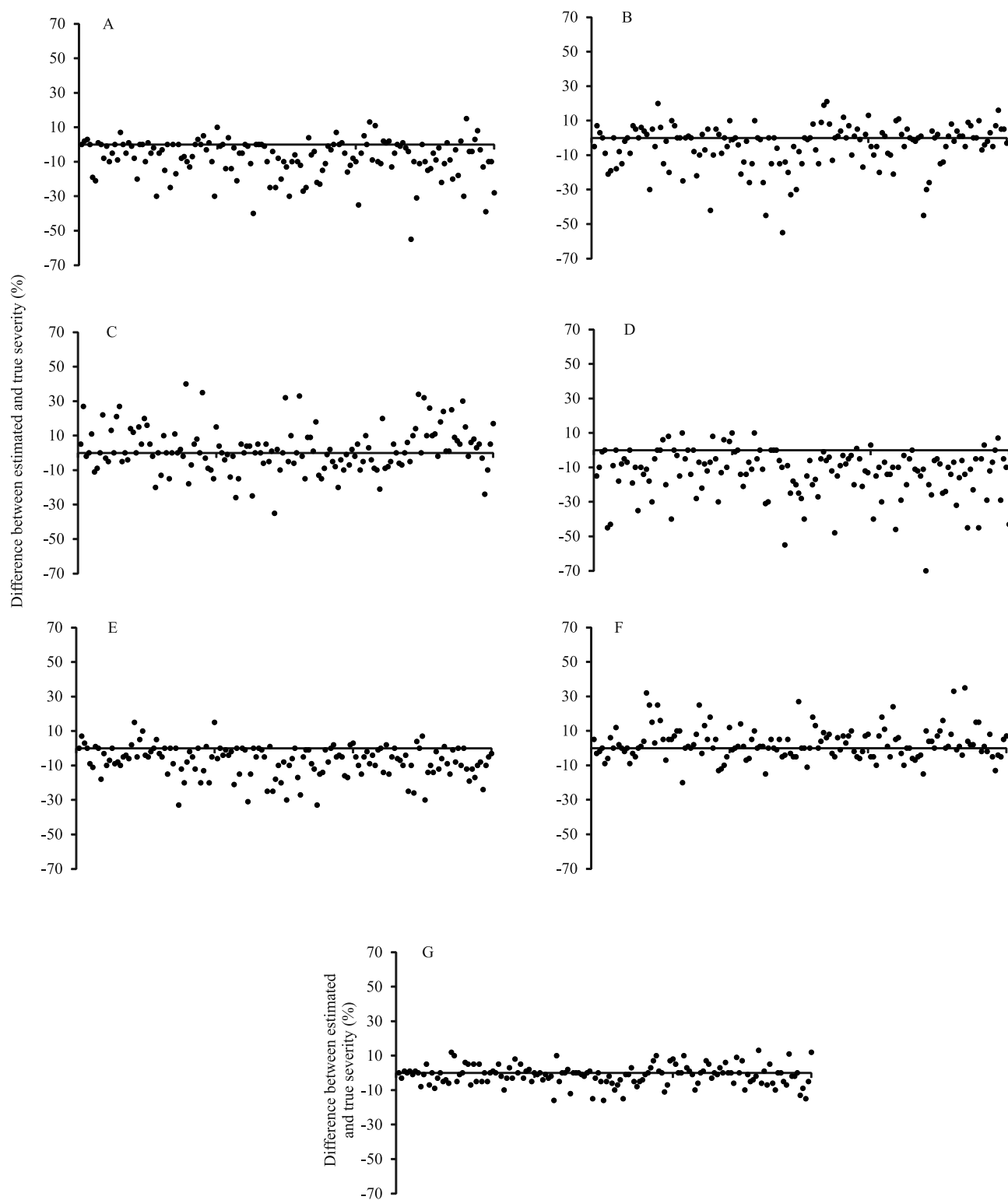
Figure 4. Distribution of the absolute errors (the estimated severity minus the true severity) of severity estimates of the postharvest physiological deterioration in cassava roots, as obtained by seven evaluators (inexperienced: 1, A; 2, B; 3, C; and 4, D; experienced: 5, E; 6, F; and 7, G) without the aid of the diagrammatic scale.
