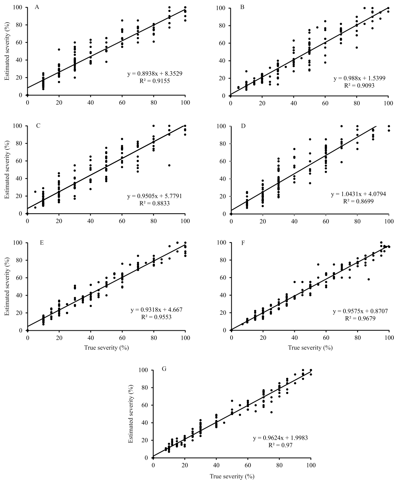
Figure 3. Relationship between the true severity and the estimated severity for the postharvest physiological deterioration in cassava roots, according to estimates by seven evaluators (inexperienced: 1, A; 2, B; 3, C; and 4, D; experienced: 5, E; 6, F; and 7, G) using the diagrammatic scale.
