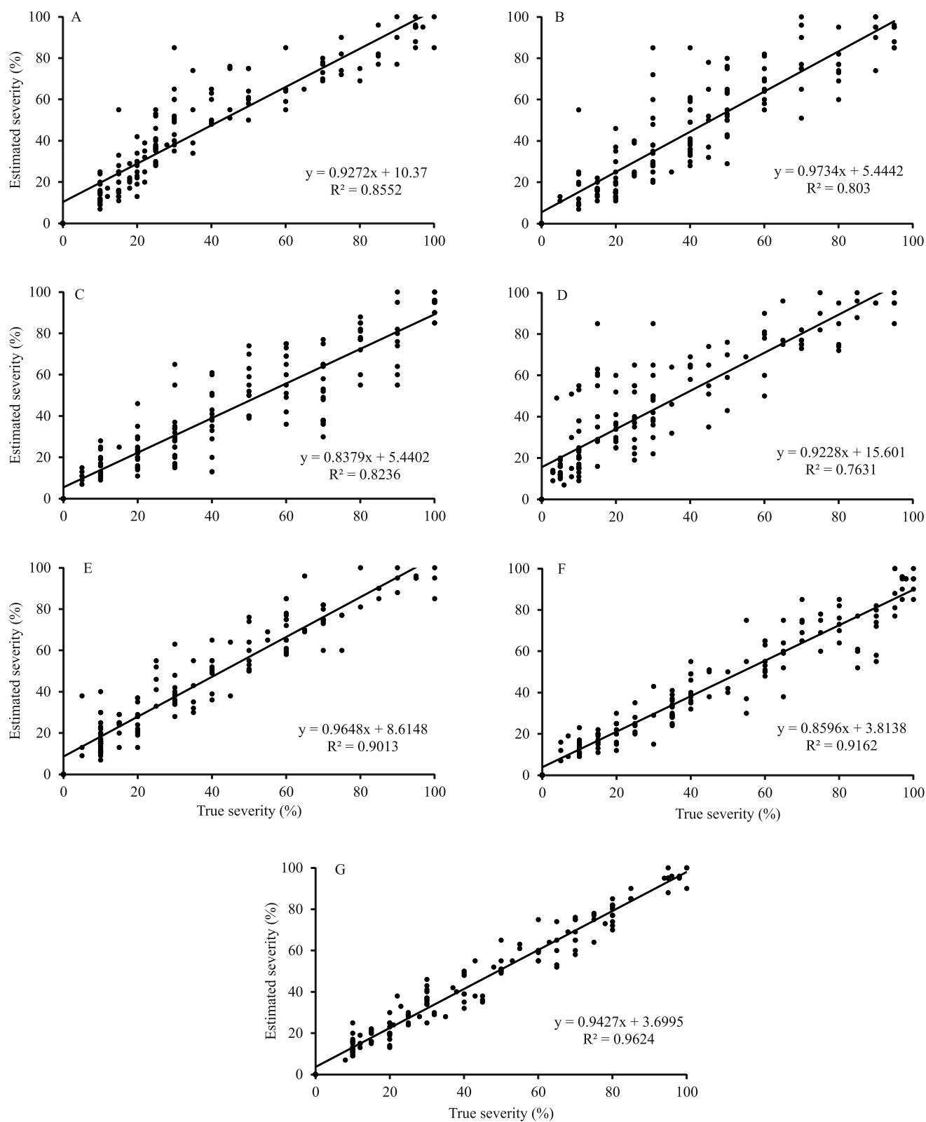
Figure 2. Relationship between the true severity and the estimated severity of the postharvest physiological deterioration in cassava roots, according to estimates by seven evaluators (inexperienced: 1, A; 2, B; 3, C; and 4, D; experienced: 5, E; 6, F; and 7, G) without the aid of diagrammatic scale.
